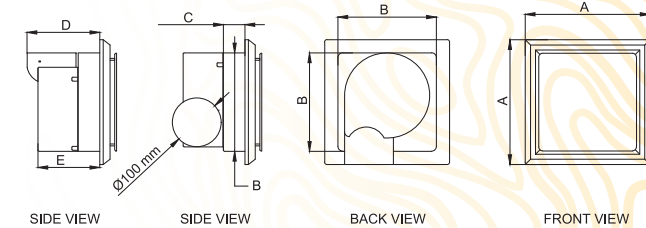
DIMENSIONS (mm)
